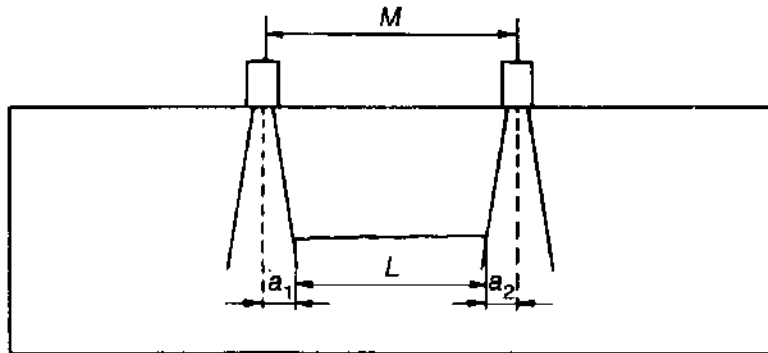
(e) M = Probe movement L = actual discontinuity size
