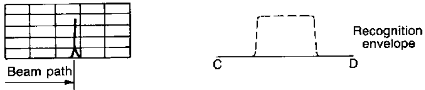
Probe movement C to D
