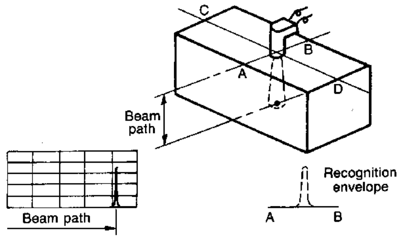
Probe movement A to B
