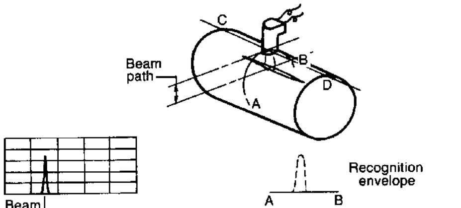
Probe movement A to B
