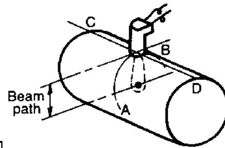
(a) Rectangular forging
