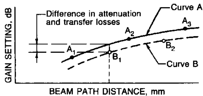
(c) Comparison of attenuation curves
