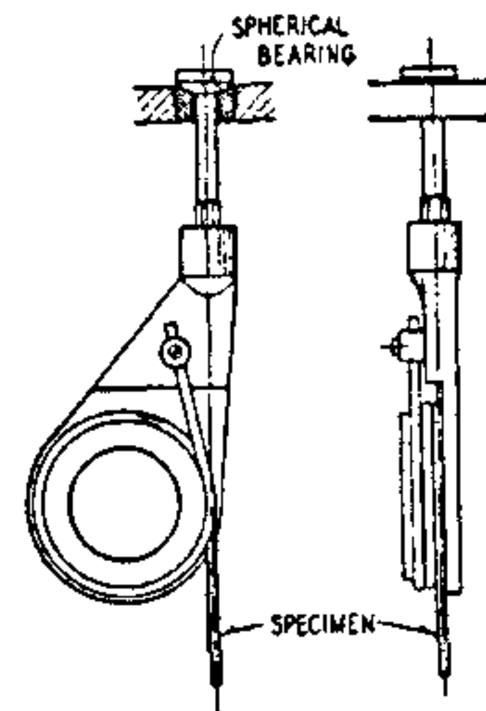
FIG. A4.2 Snubbing-Type Gripping Device
