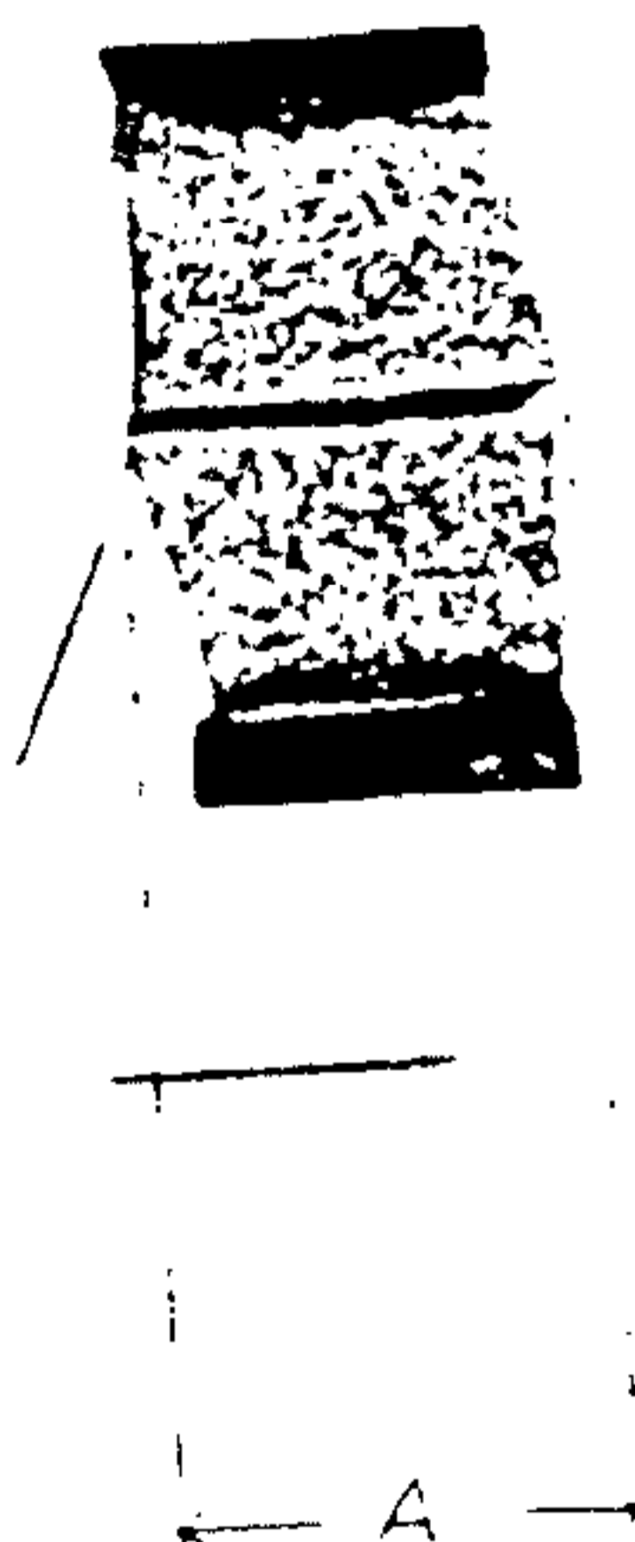
FIG. 15 Halves of Broken Charpy V-Notch Impact Specimen Joined for the Measurement of Lateral Expansion, Dimension A
